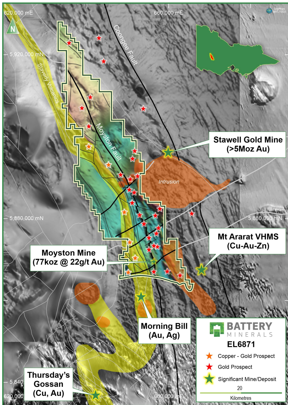
Figure 3: Stavelly Stawell Au- Cu Project
